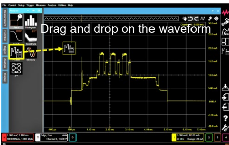
Figure 17. Automated power and current profiler results
