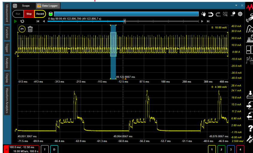
Figure 19. CX3300 can read and playback from the storage for deep analysis similar to the scope mode
