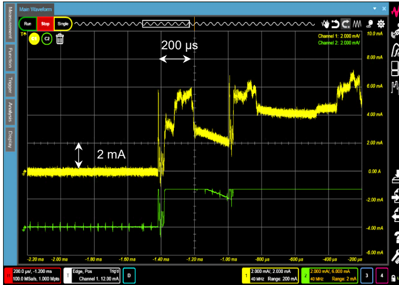
Figure 9. CX1101A measurement example
