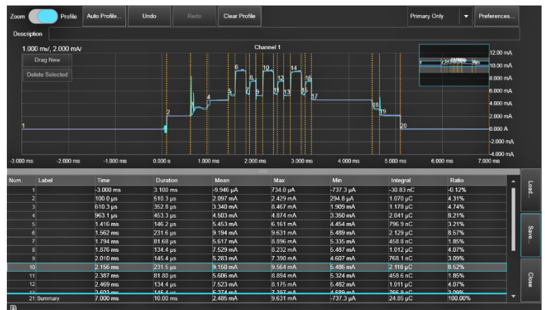
Figure 17. Automated power and current profiler results
